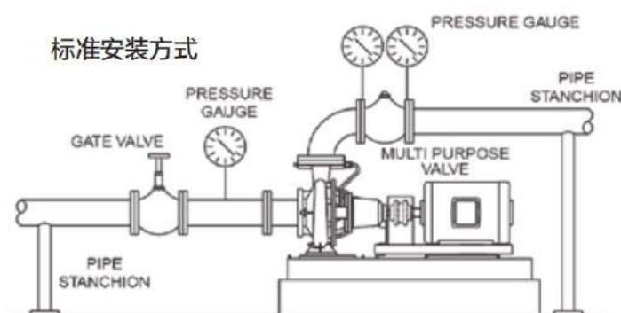
Fig. 3 - Typical Installation - Horizontal Piping
